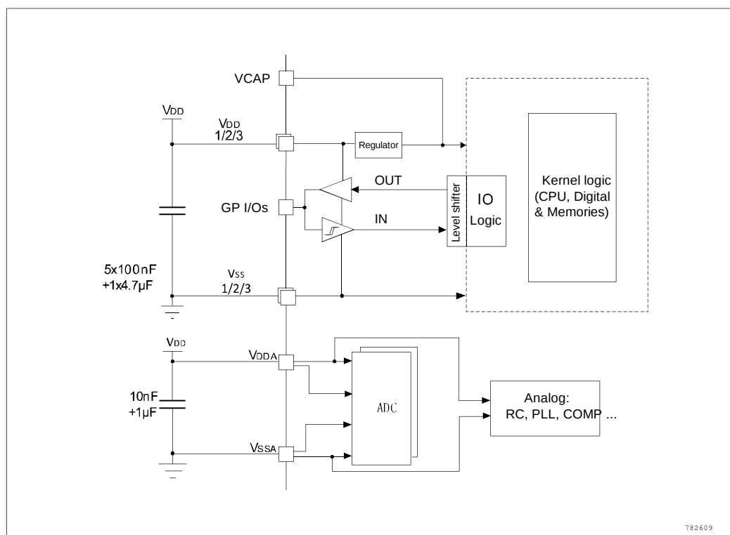
Figure 7. Power scheme
