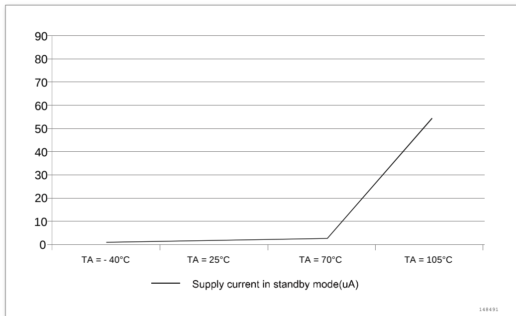
Figure 9. Typical current consumption in standby mode vs. temperature at V_{DD} = 3.3\text{V}
