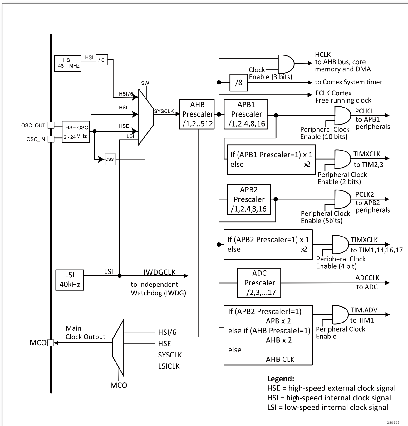
Figure 2. Clock tree
