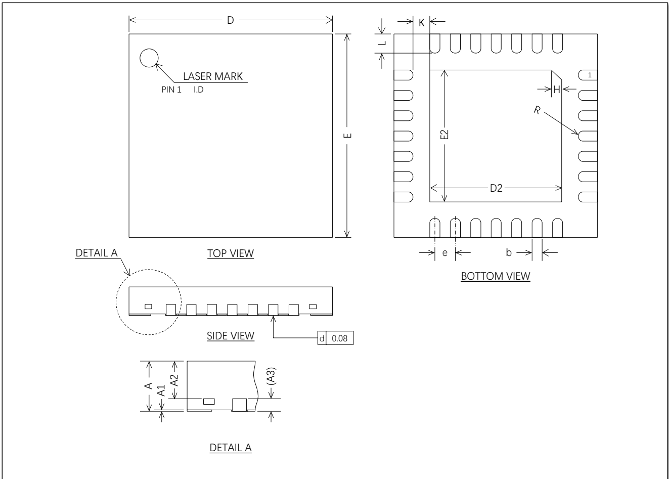
Figure 6-4 QFN28 package dimension
