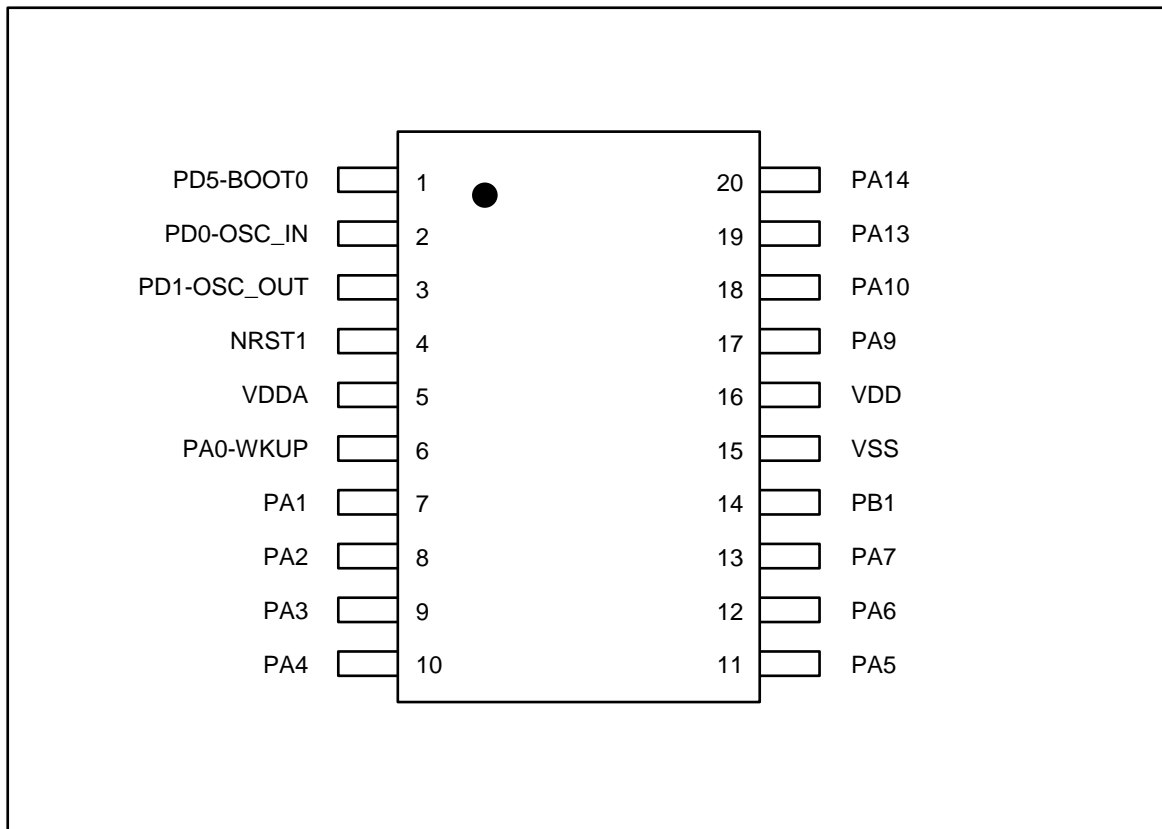
Figure 4-5 TSSOP20 pinout diagram
