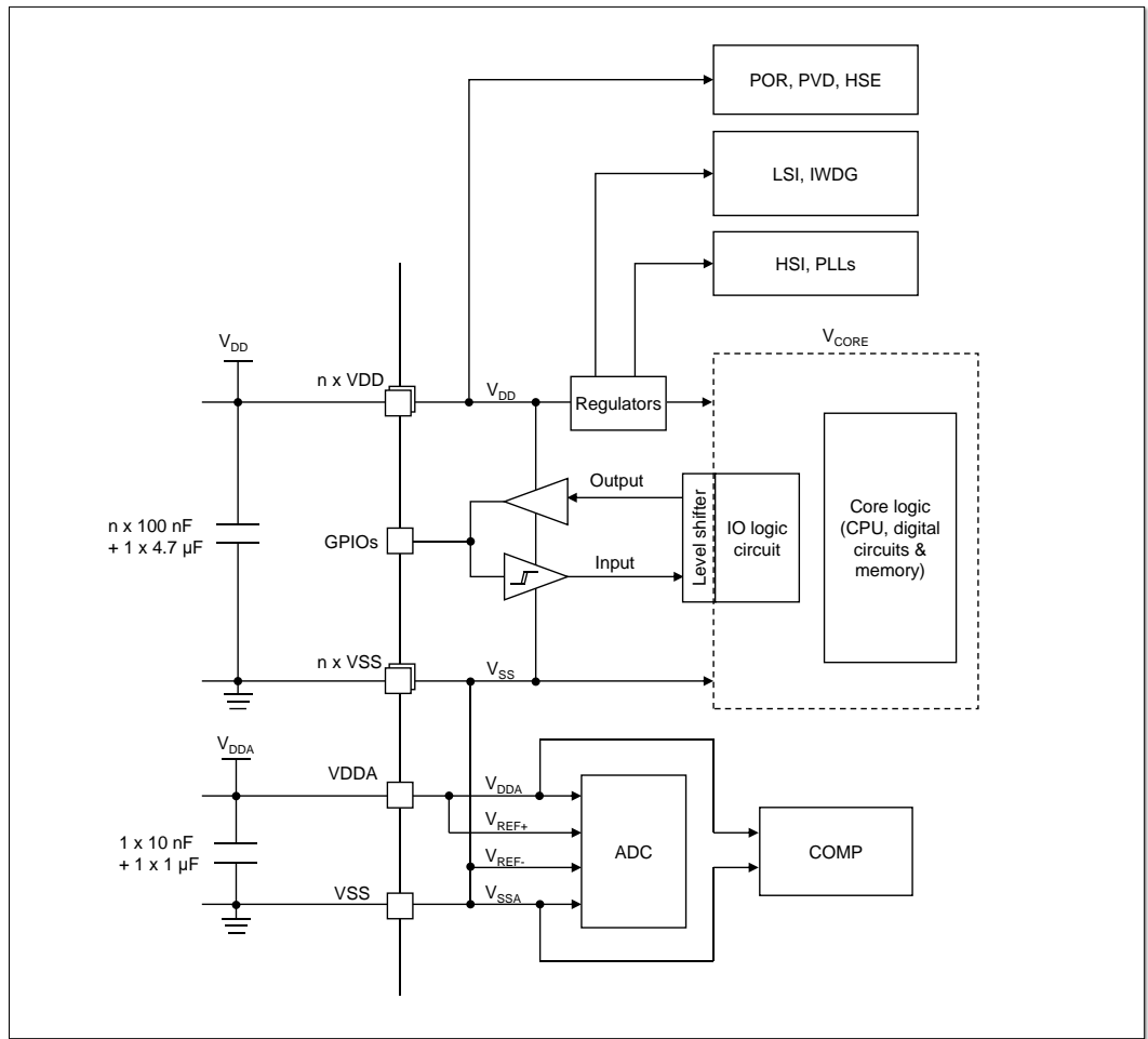
Figure 5-3 Power scheme
