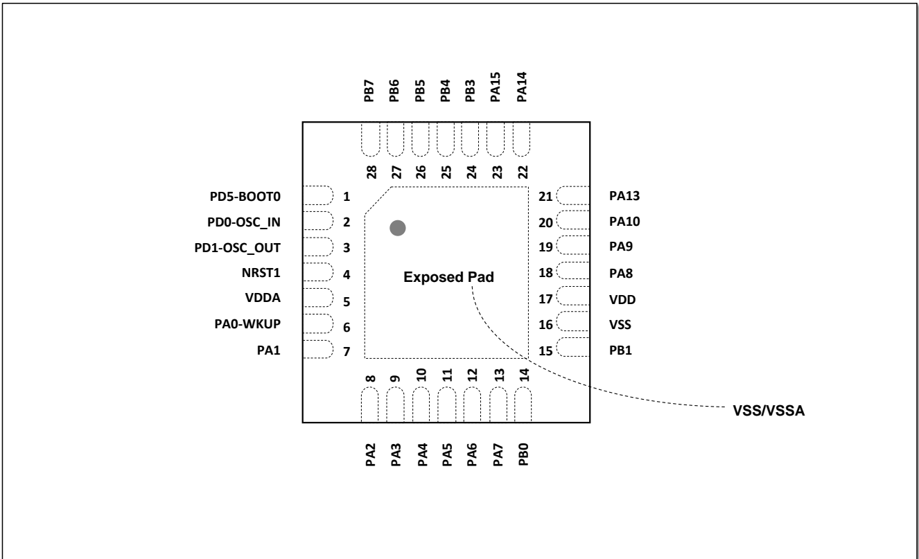
Figure 4-4 QFN28 pinout diagram
