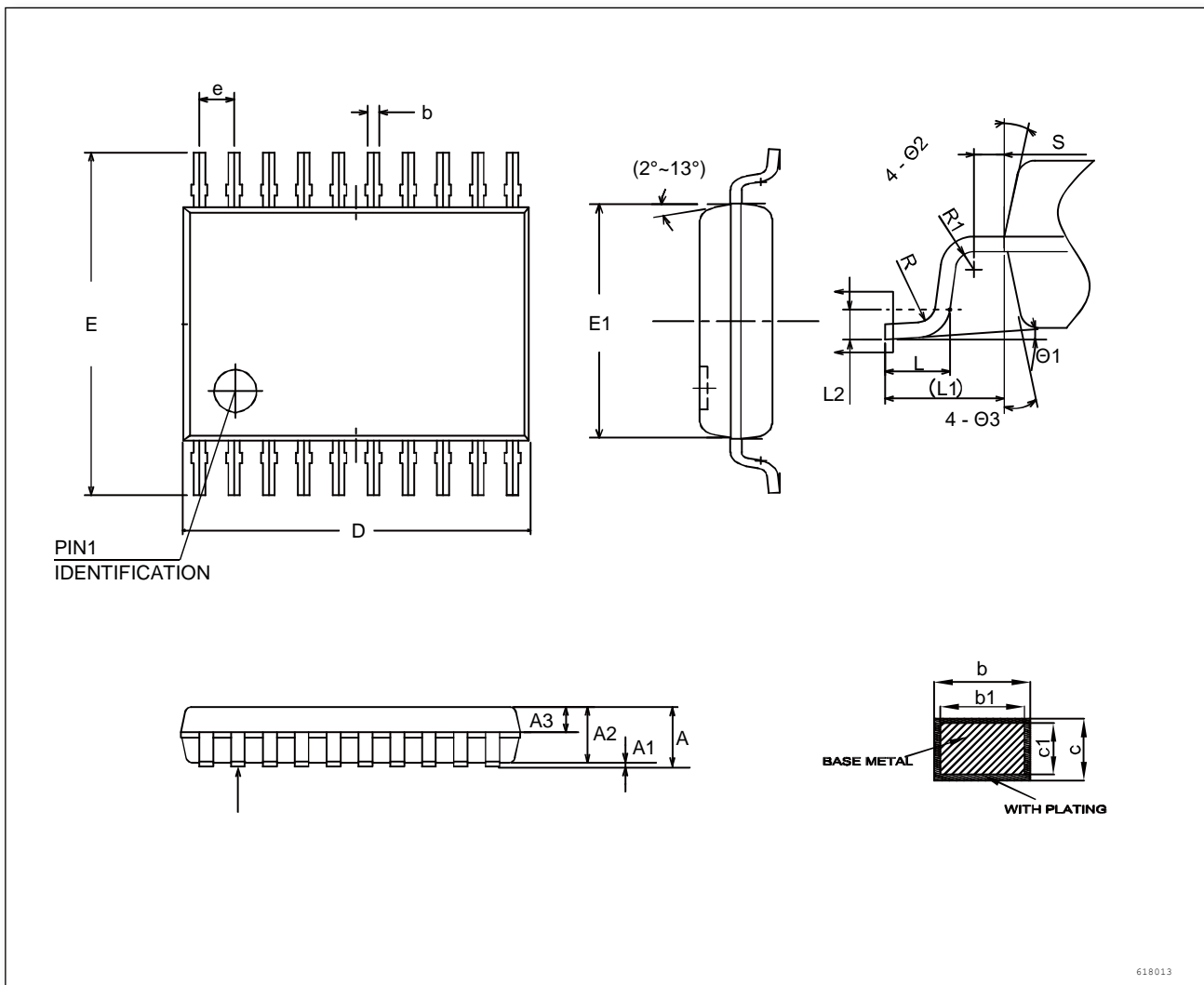
Figure 6-5 TSSOP20 package dimension
