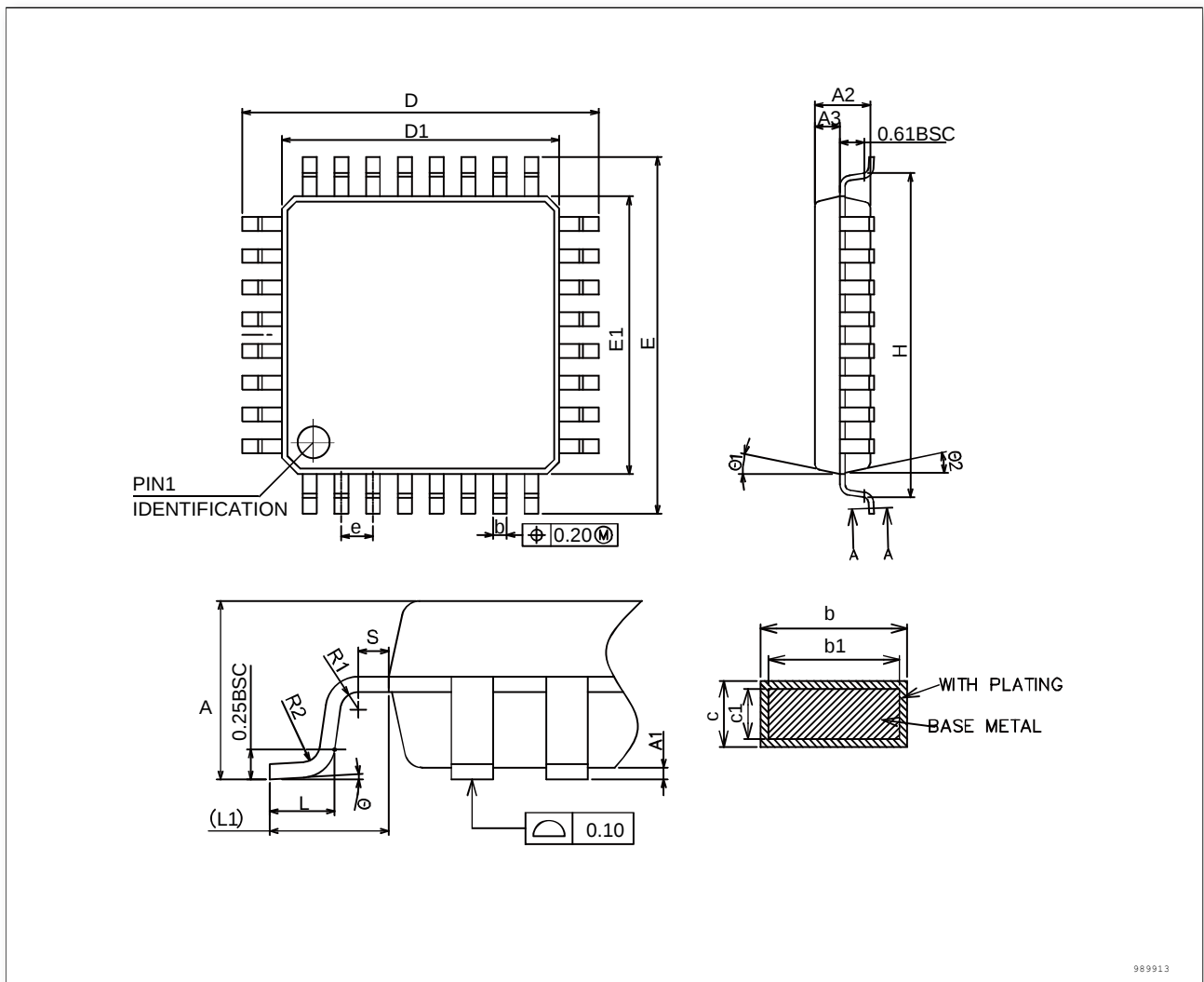
Figure 6-2 LQFP32 package dimension
