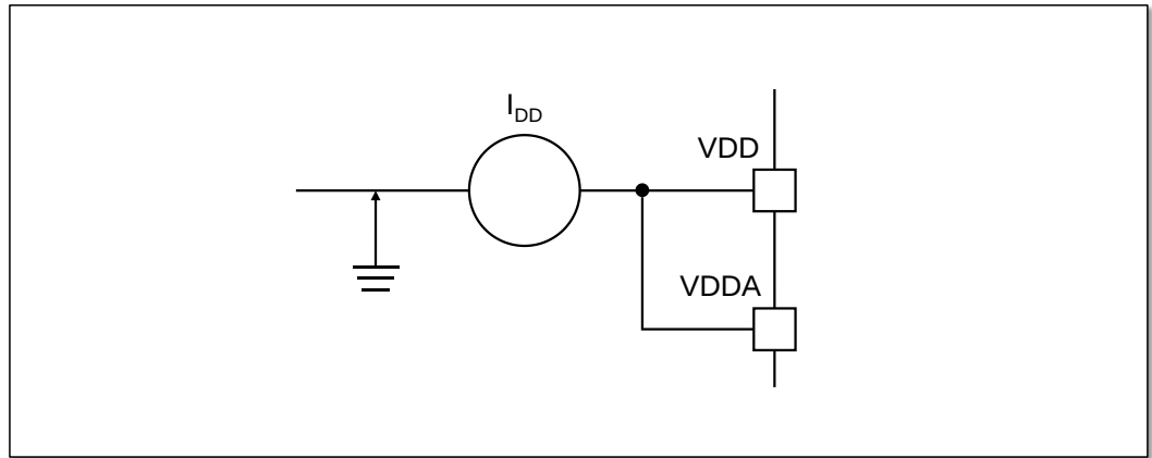
Figure 5-4 Current consumption measurement scheme
