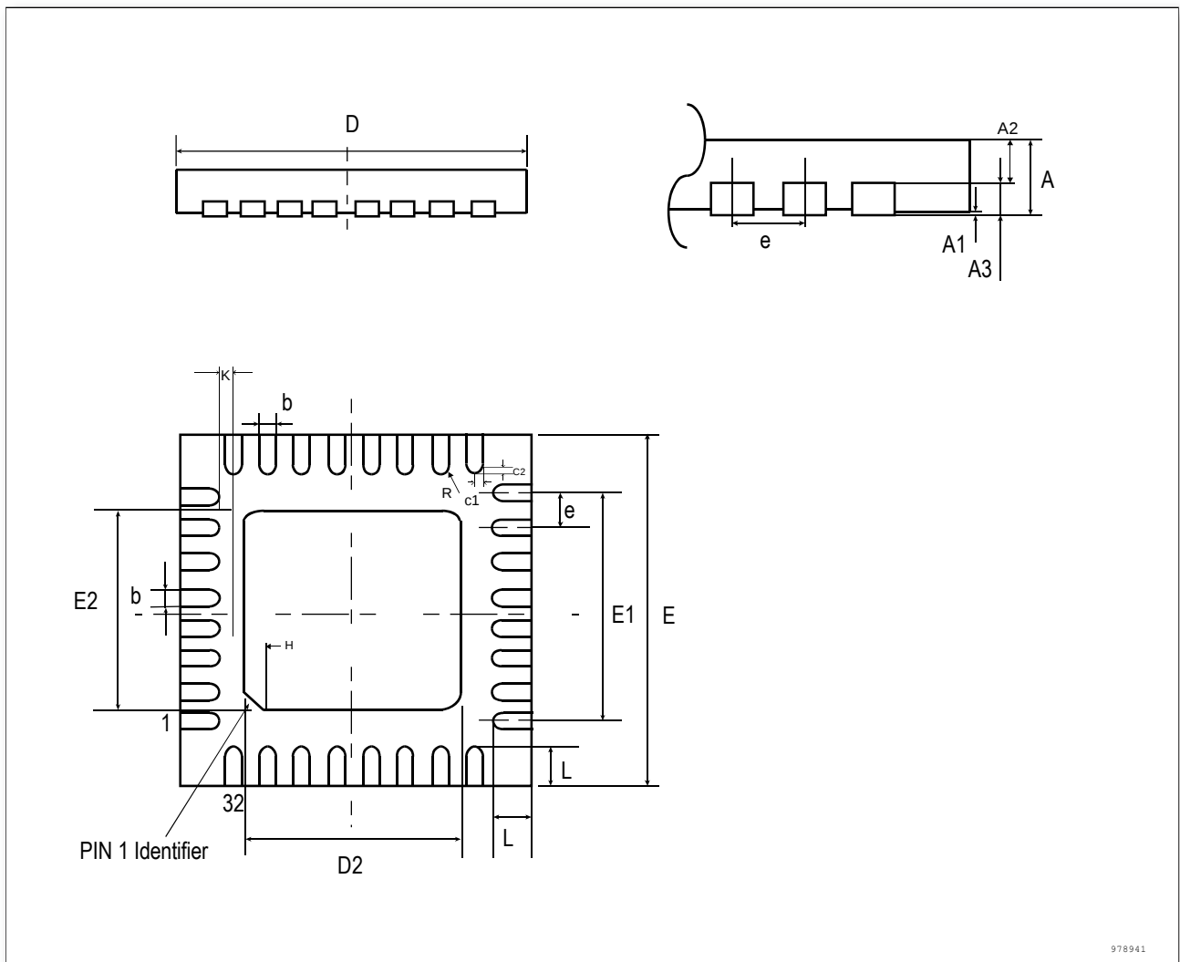
Figure 6-3 QFN32 package dimension
