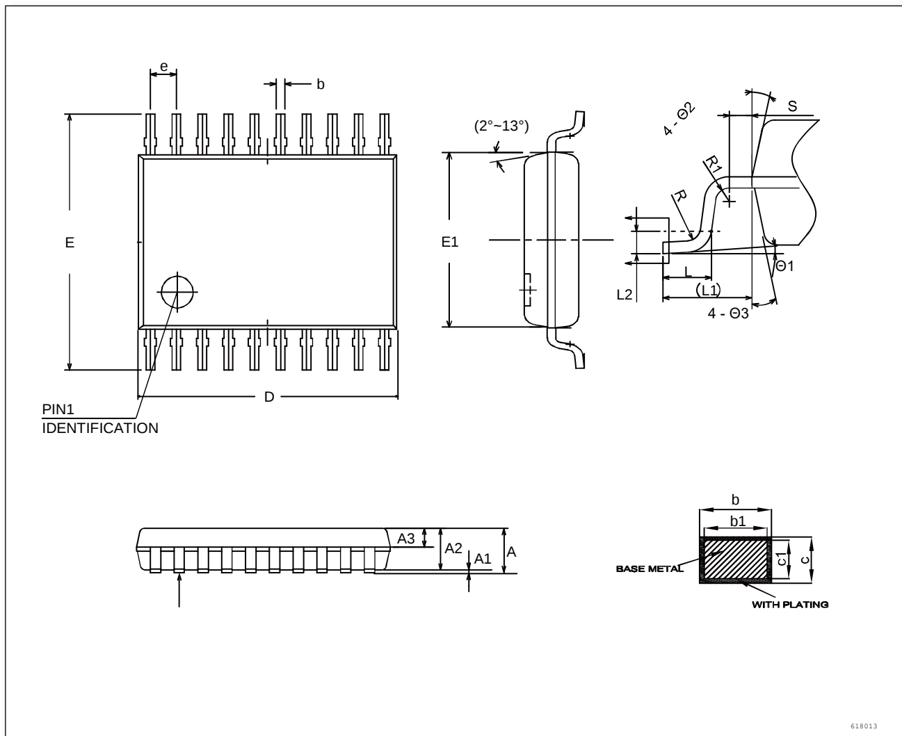
Figure 6-4 TSSOP20 package dimension
