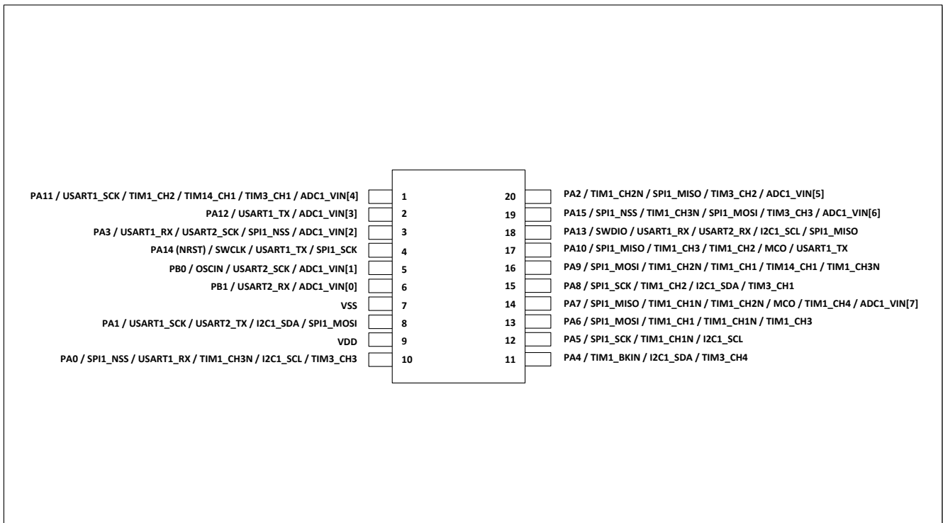
Figure 4-2 TSSOP20 pinout diagram
