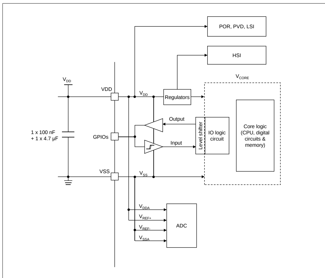
Figure 5-3 Power scheme (1)
