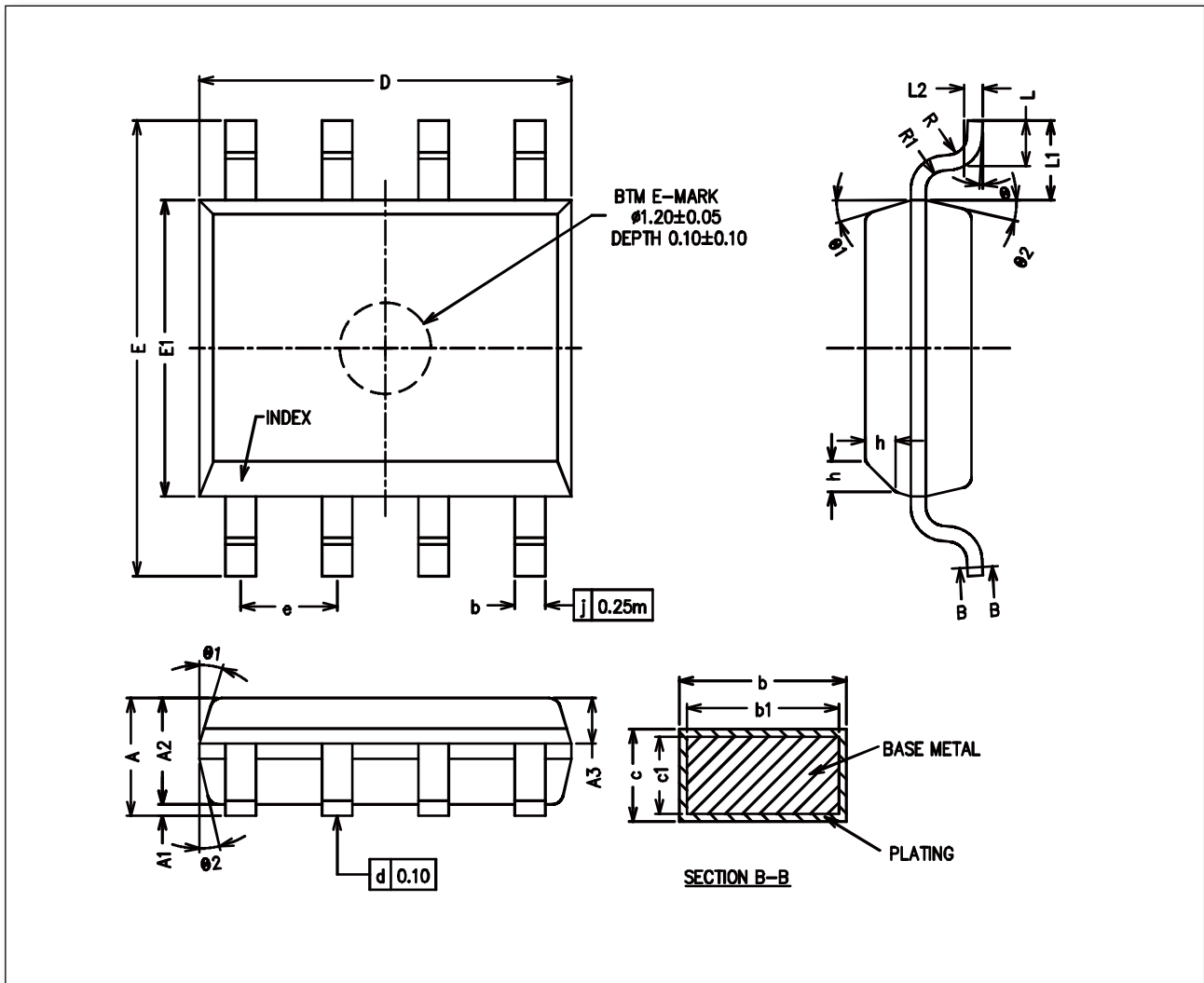
Figure 6-3 SOP8 package dimension
