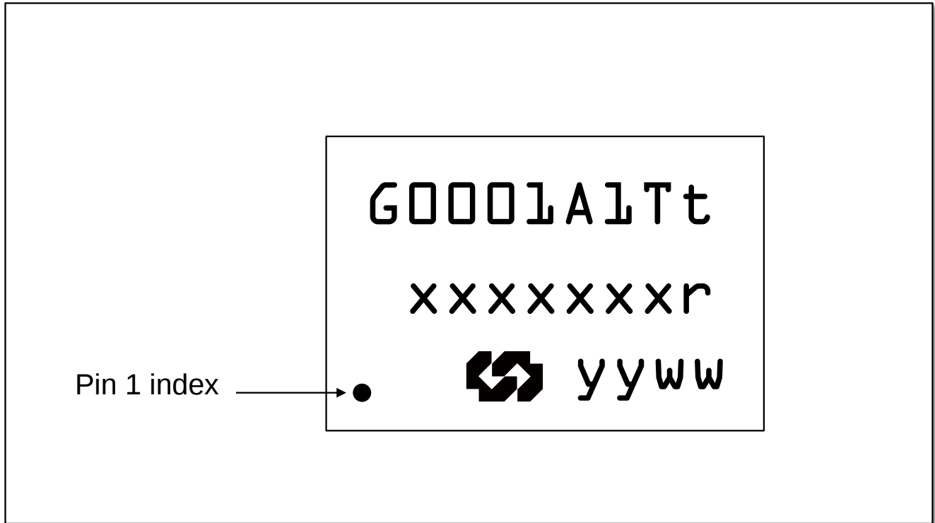
Figure 2-1 TSSOP20 package marking
