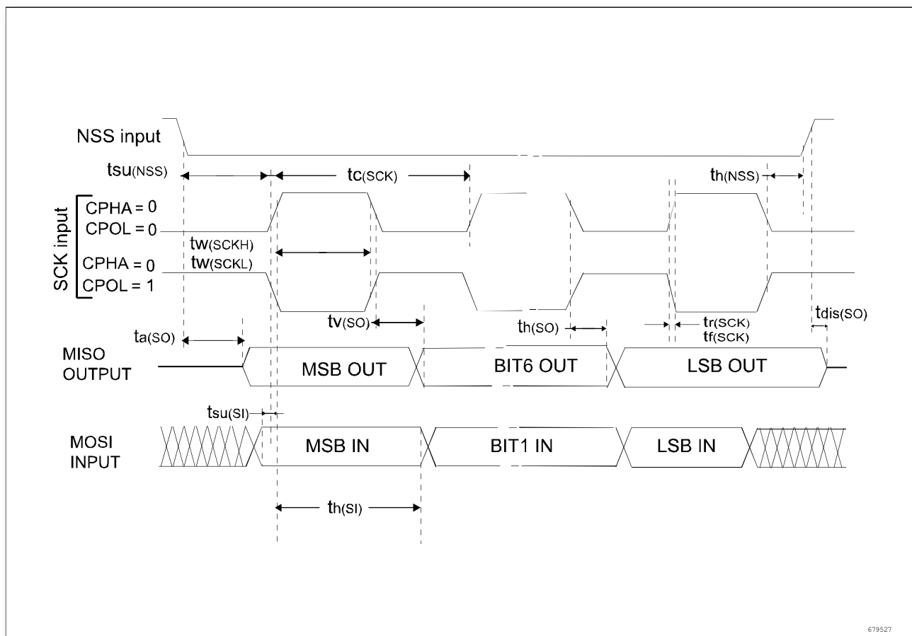
Figure 5-9 SPI timing diagram-slave mode and CPHA = 0, CPHASEL = 1
