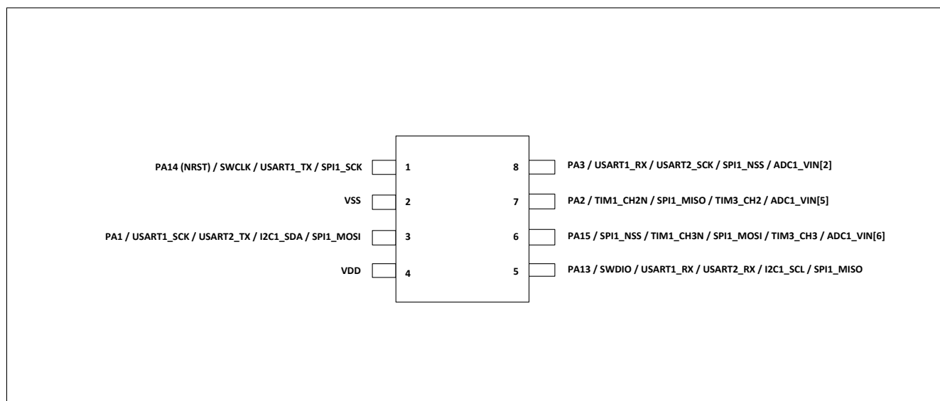
Figure 4-3 SOP8 – type 0 pinout diagram
