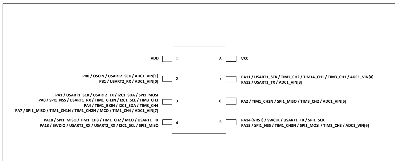
Figure 4-4 SOP8 – type 1 pinout diagram
