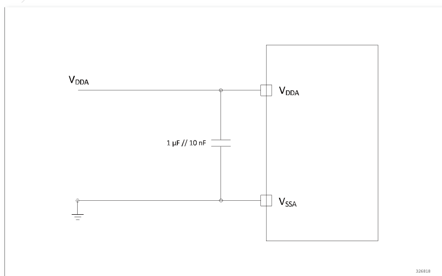
Figure 5-14 Power supply and reference power supply decoupling circuit
