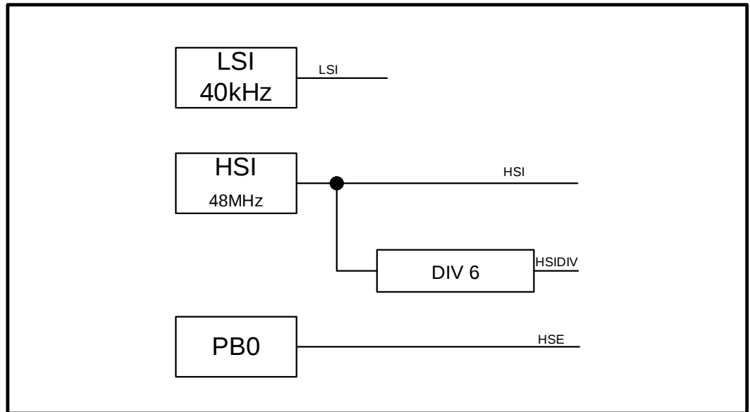
Figure 3-2 System clock sources
