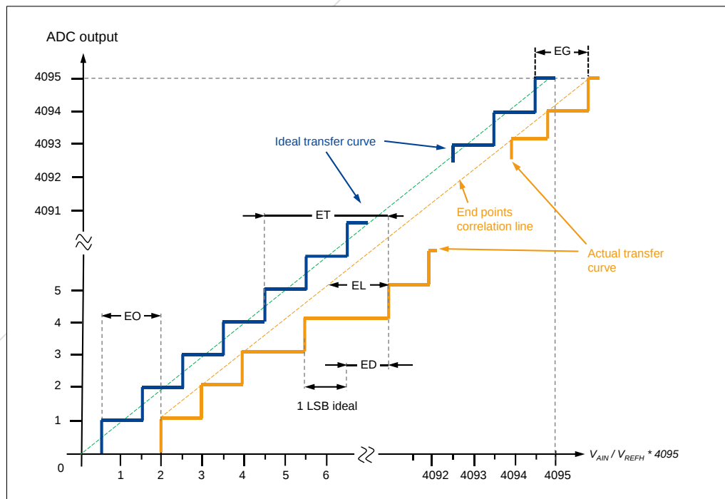
Figure 5-12 Schematic diagram of ADC static parameters
