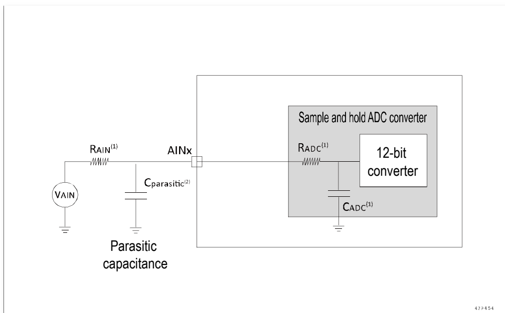
Figure 5-13 Typical connection diagram using the ADC
