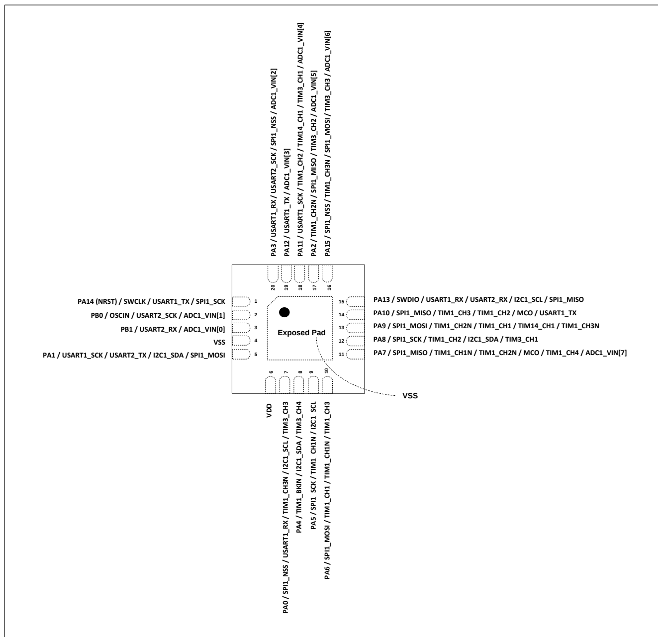
Figure 4-1 QFN20 pinout diagram
