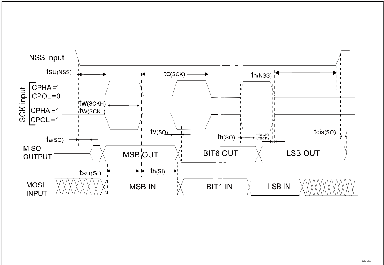
Figure 5-10 SPI timing diagram-slave mode and CPHA = 1, CPHASEL = 1 (1)
