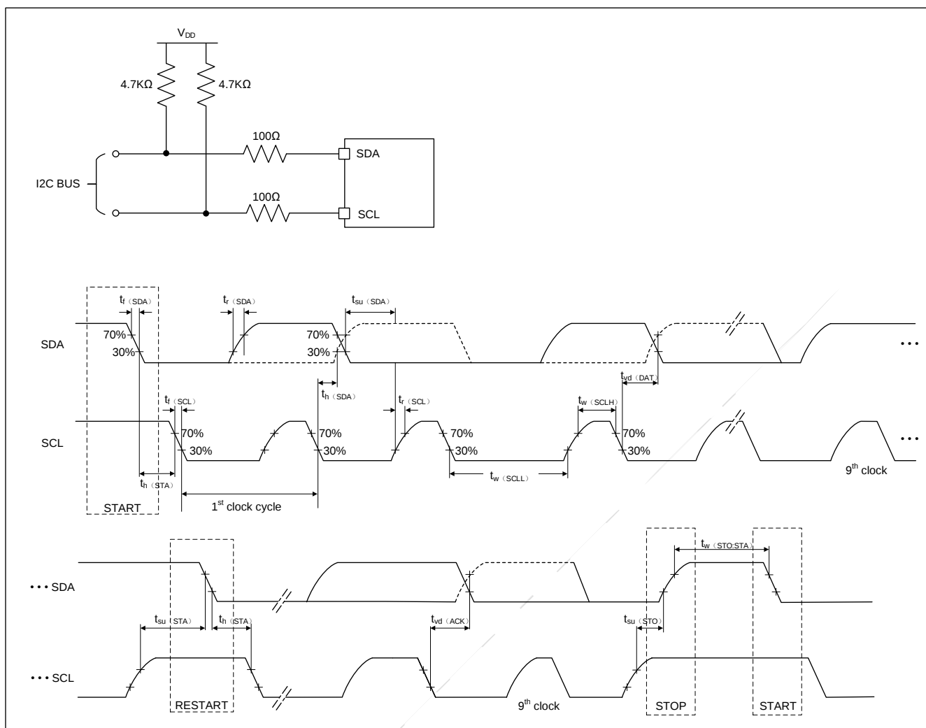
Figure 5-8 I2C bus AC waveform and measurement circuit (1)
