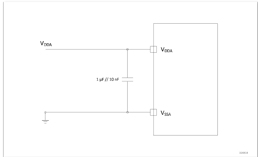
Figure 5-14 Power supply and reference power supply decoupling circuit
