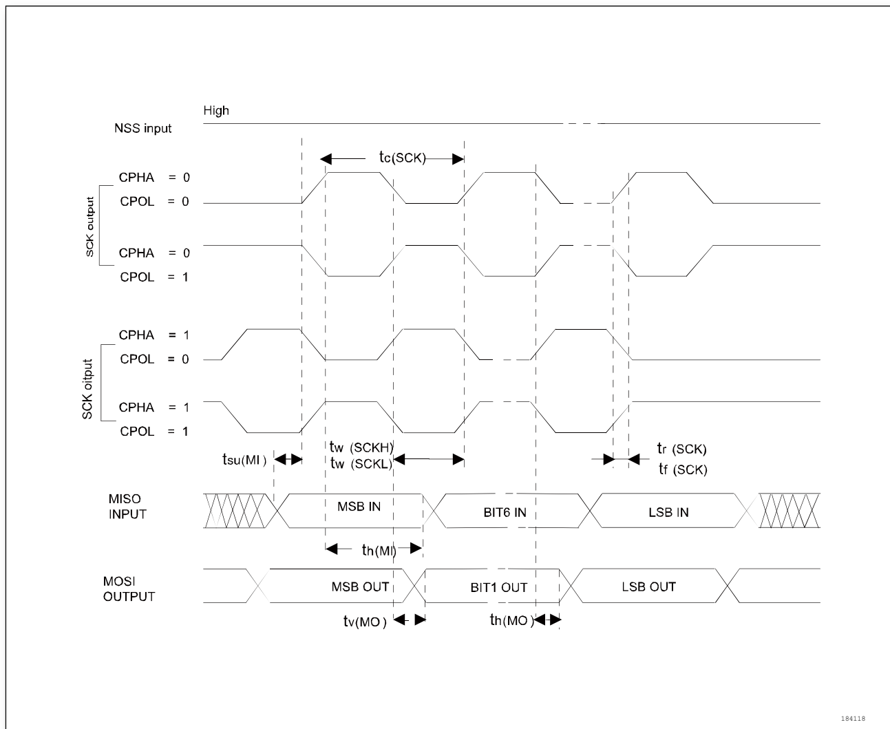
Figure 5-11 SPI timing diagram-master mode, CPHASEL = 1 (1)
