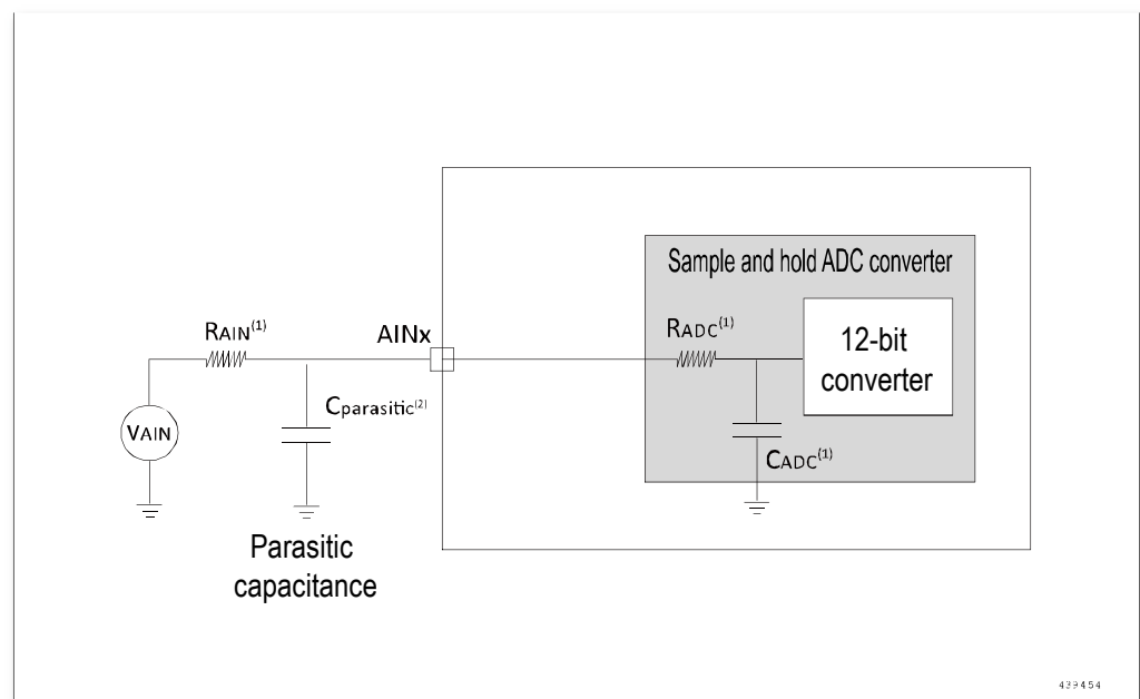
Figure 5-13 Typical connection diagram using the ADC
