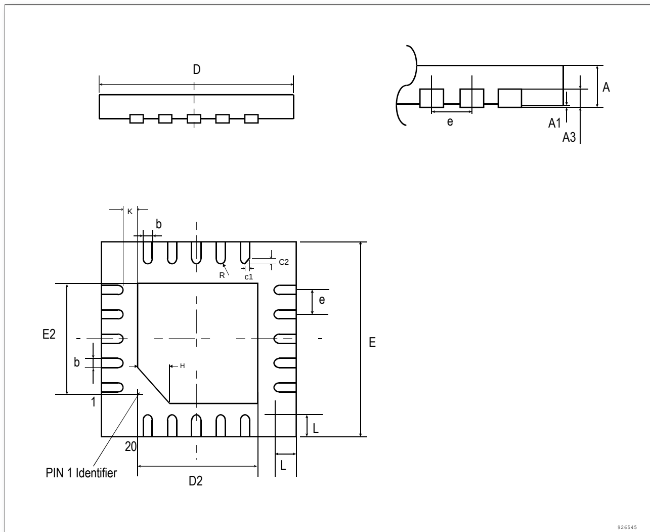
Figure 6-1 QFN20 package dimension
