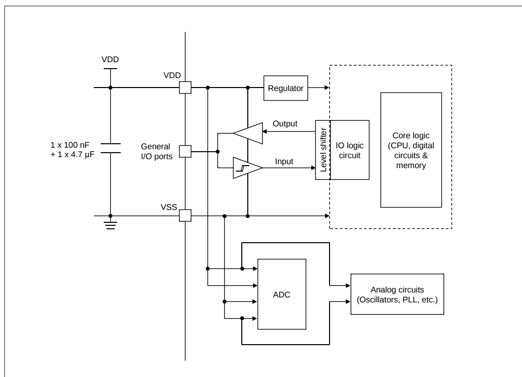
Figure 5-3 Power scheme (1)
