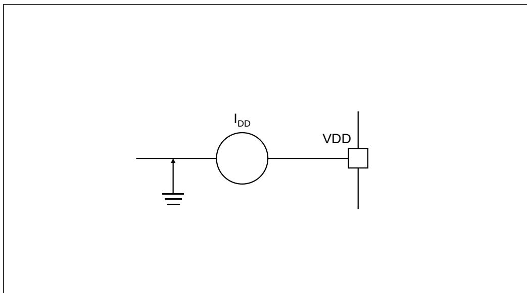
Figure 5-4 Current consumption measurement scheme
