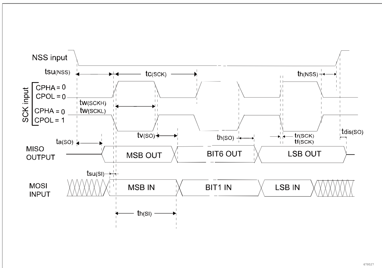
Figure 5-9 SPI timing diagram-slave mode and CPHA = 0, CPOLSEL = 1
