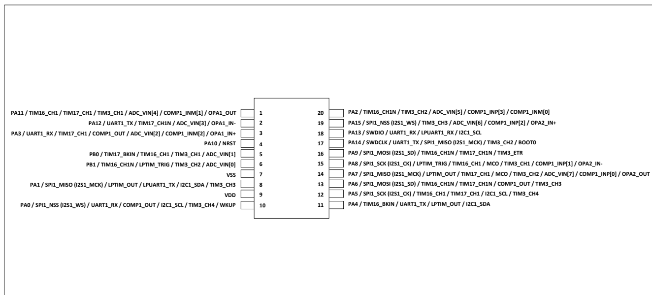
Figure 4-2 TSSOP20 pinout diagram
