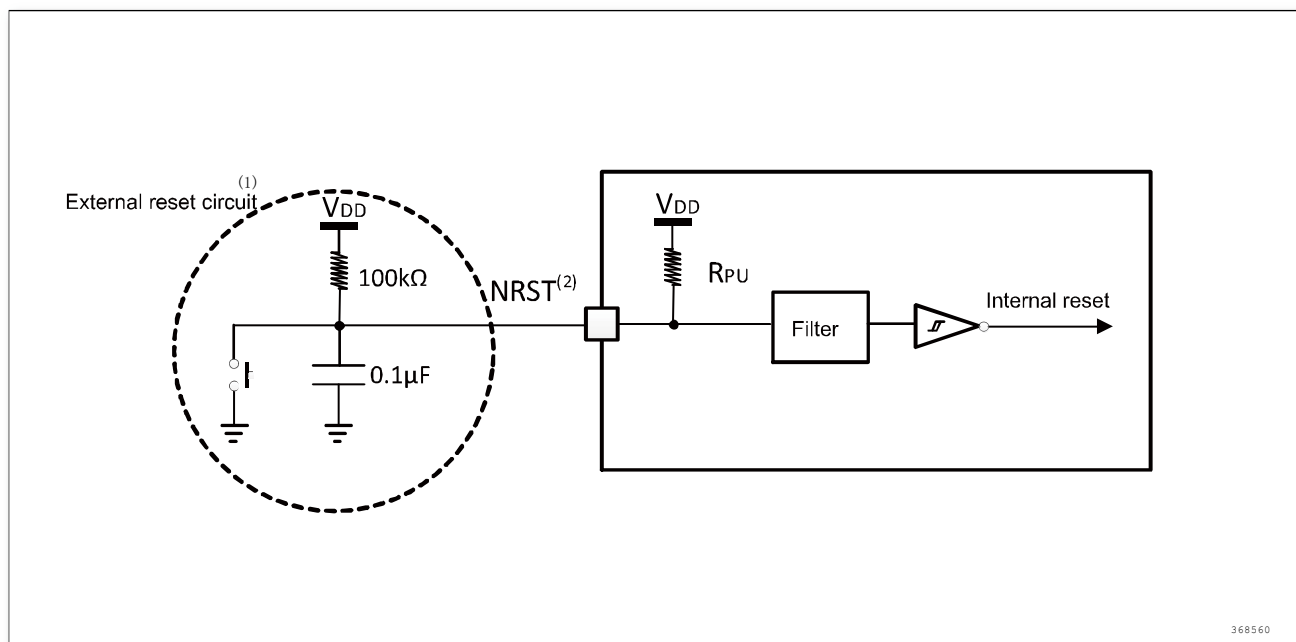
Figure 5-7 Recommended NRST pin protection
