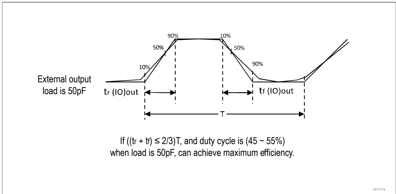
Figure 5-6 I/O AC characteristics
