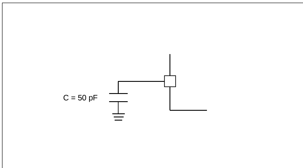
Figure 5-1 Load condition of the pin
