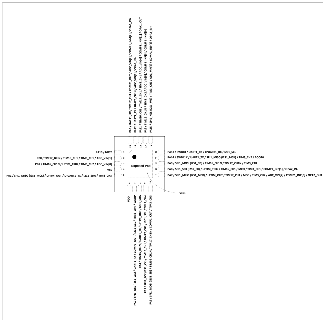
Figure 4-1 QFN20 pinout diagram
