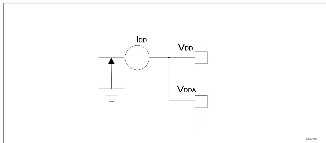
Figure 14 Current consumption measurement scheme
