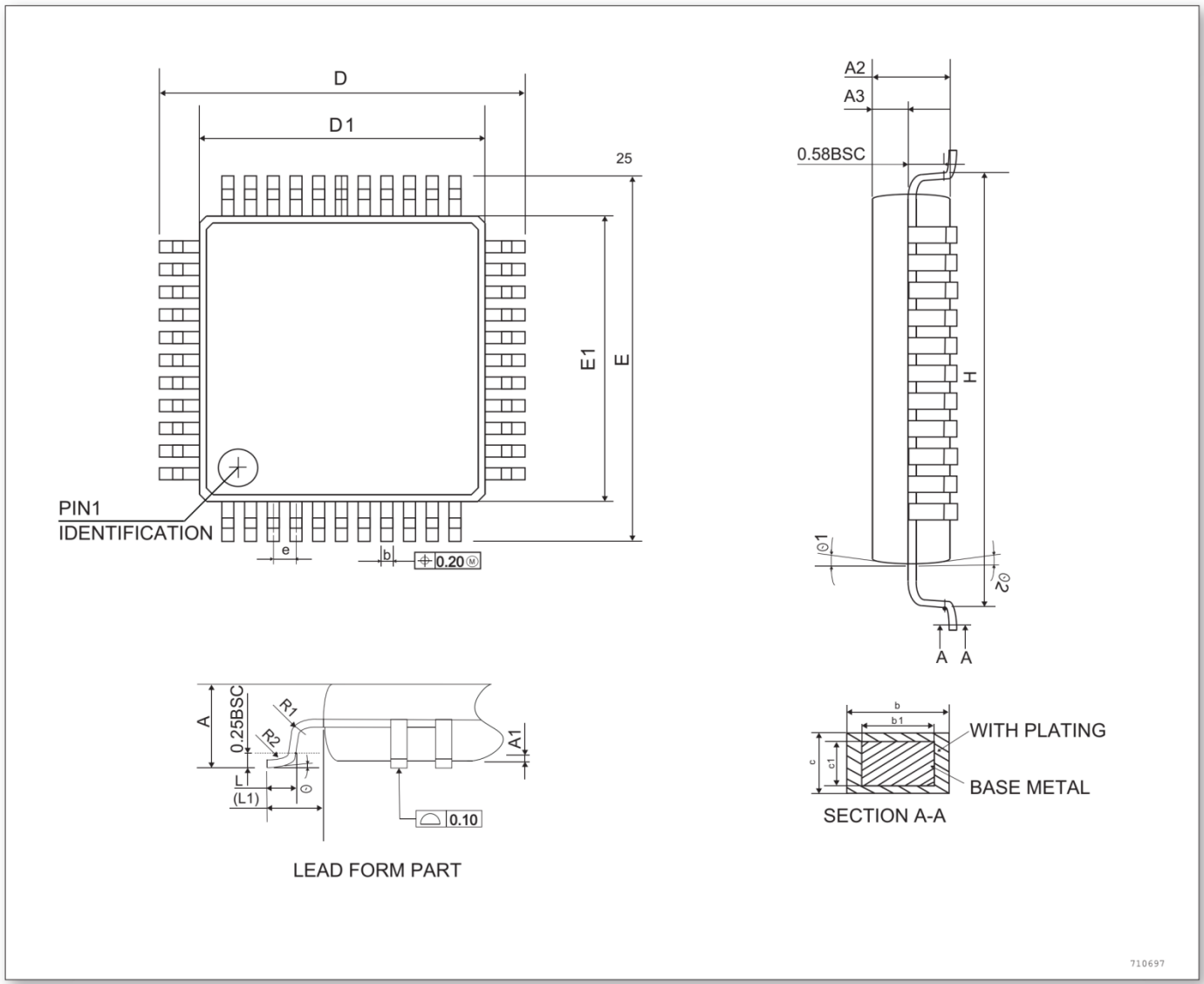
Figure 28 LQFP44, 44-pin low profile quad flat package
