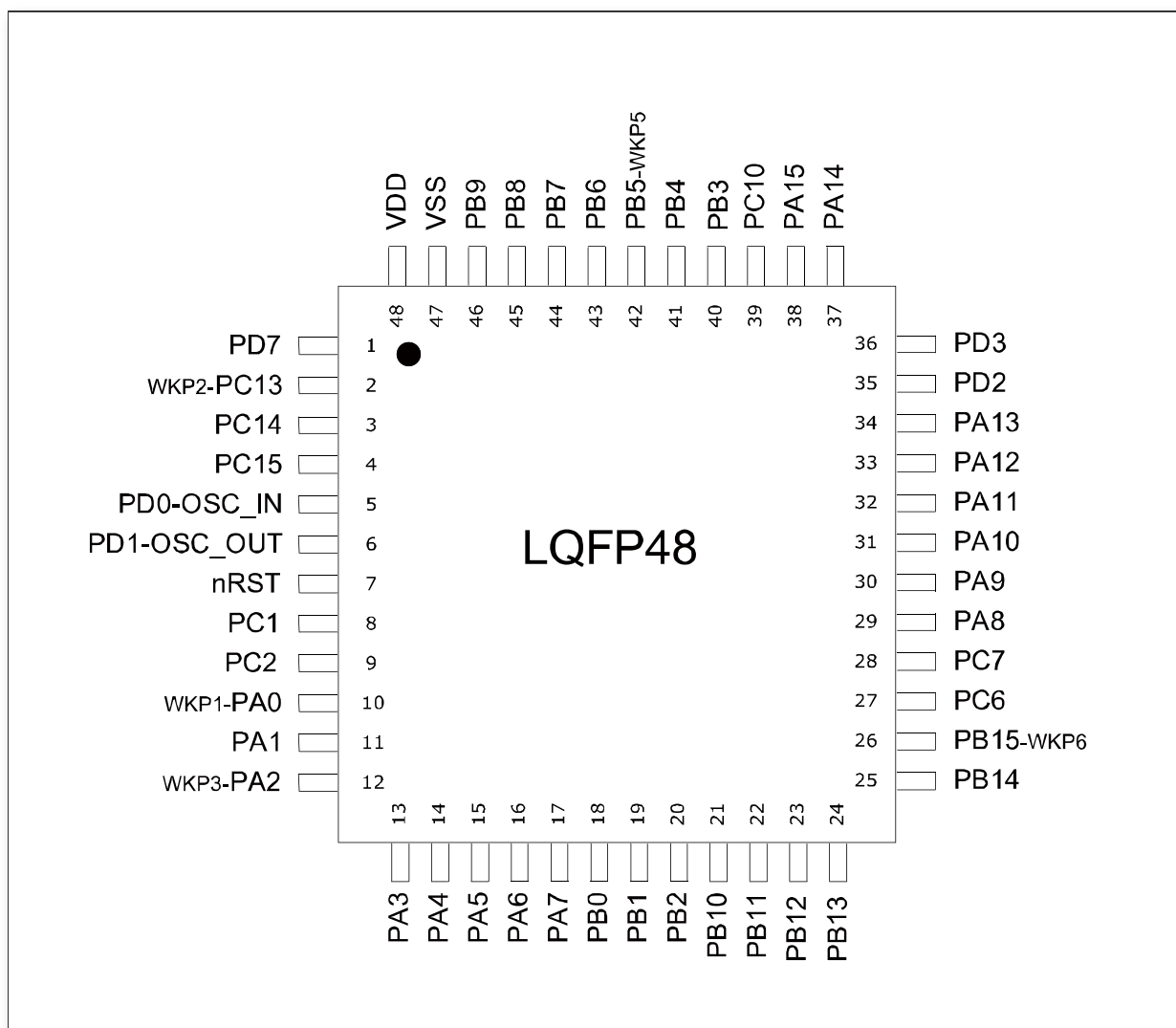
Figure 10 MM32SPINEBK Pinout diagram
