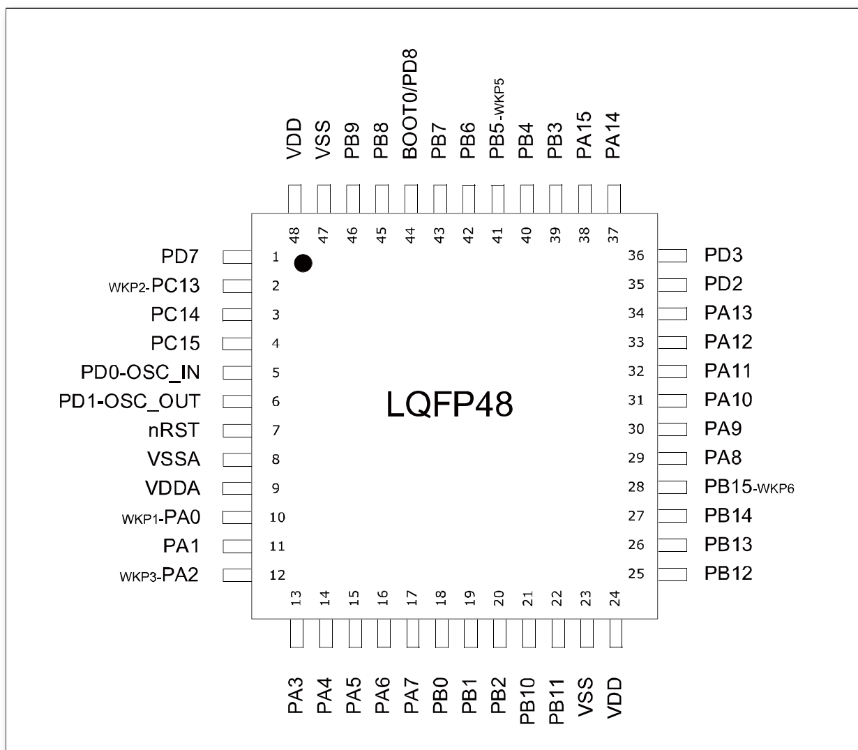
Figure 6 LQFP48 Pinout diagram
