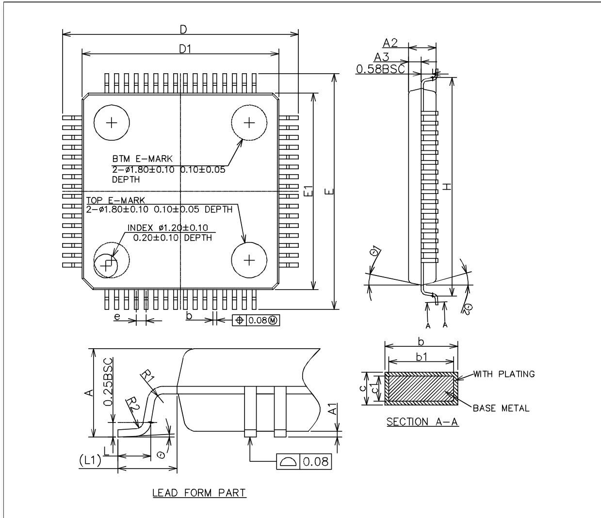
Figure 26 LQFP64, 64-pin low-profile quad flat package
