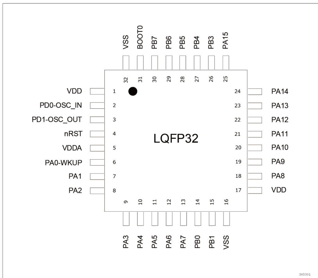
Figure 9 LQFP32 Pinout diagram
