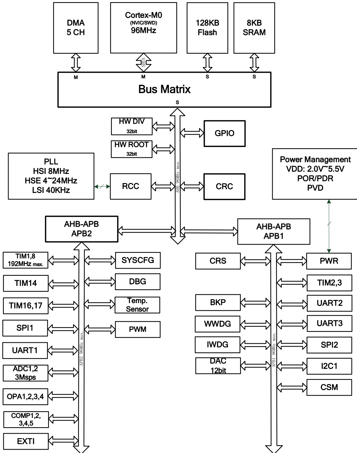
Figure 3 Block diagram
