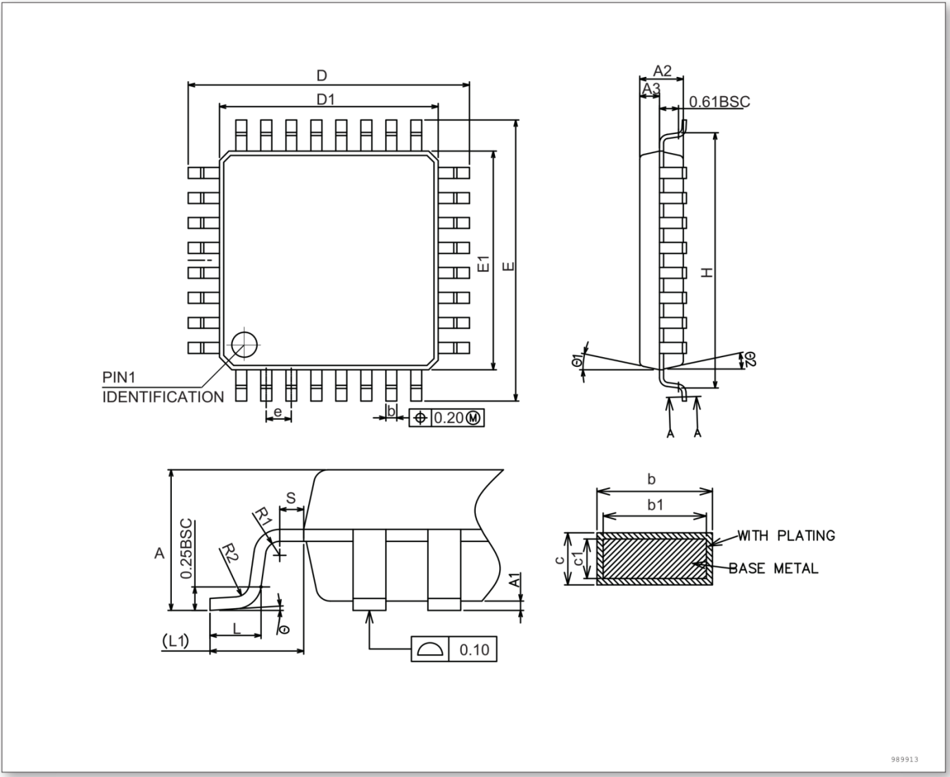
Figure 30 LQFP32, 32-pin low profile quad flat package
