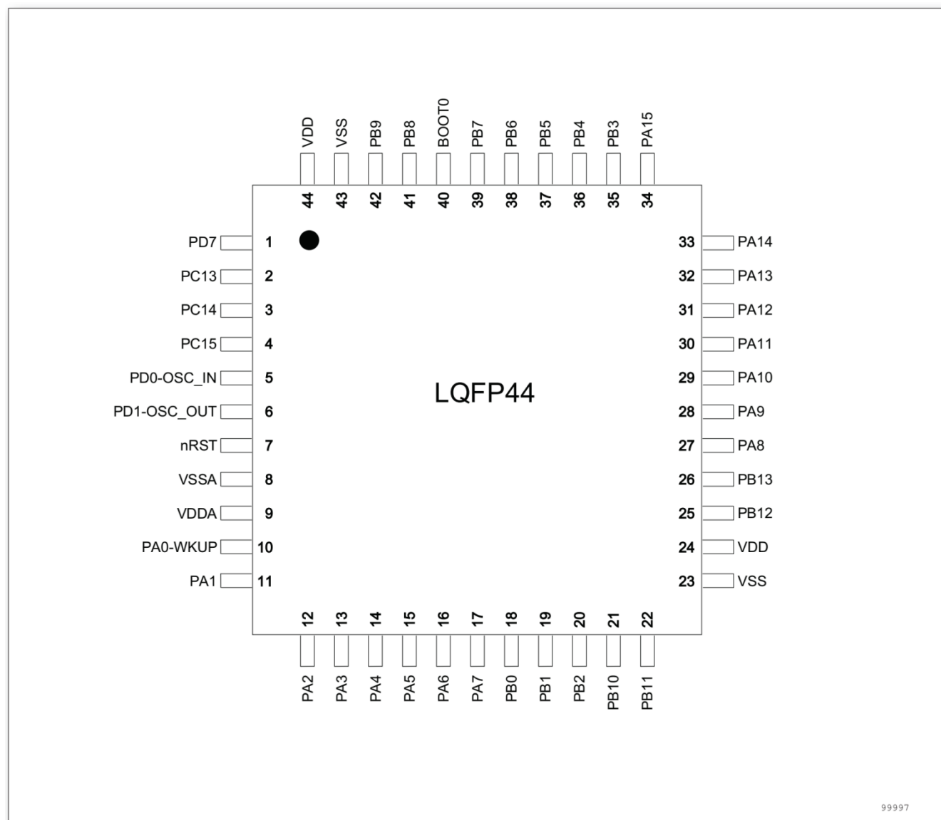
Figure 8 LQFP44 Pinout diagram
