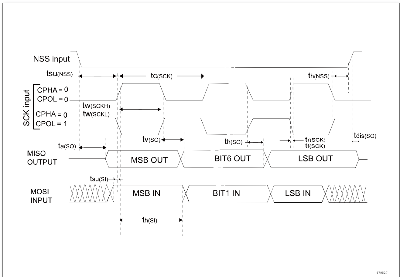
Figure 21 SPI timing diagram-slave mode and CPHA = 0, CPHASEL = 1
