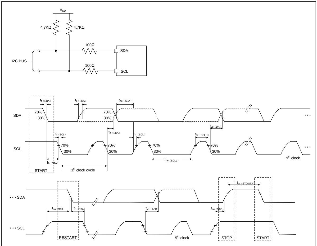
Figure 20 I2C bus AC waveform and measurement circuit (1)
