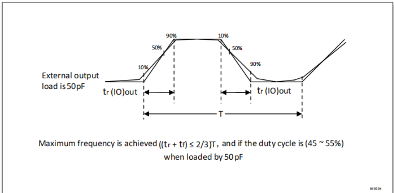
Figure 18 Input/output AC characteristics definition
