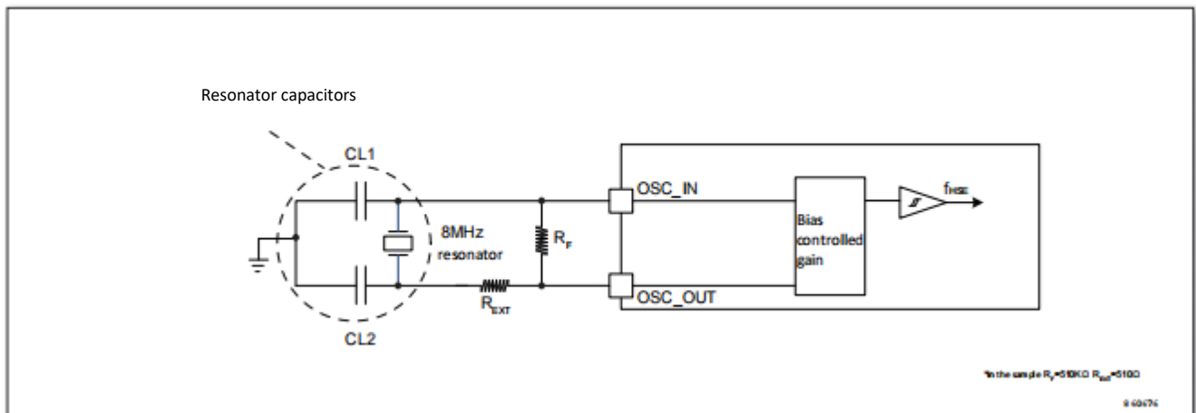
Figure 17 Typical application with an 8MHz crystal
