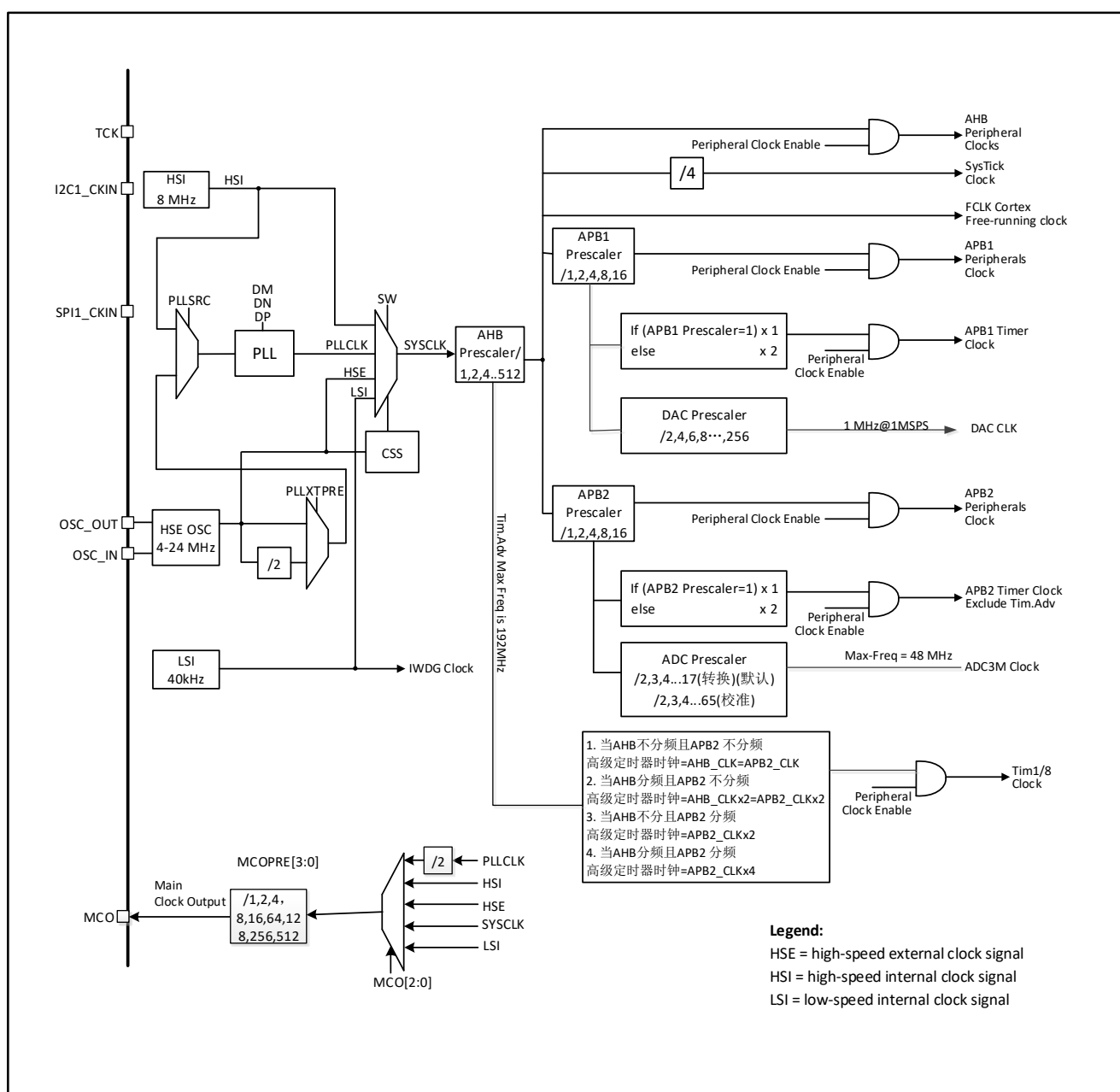
Figure 4 Clock tree
