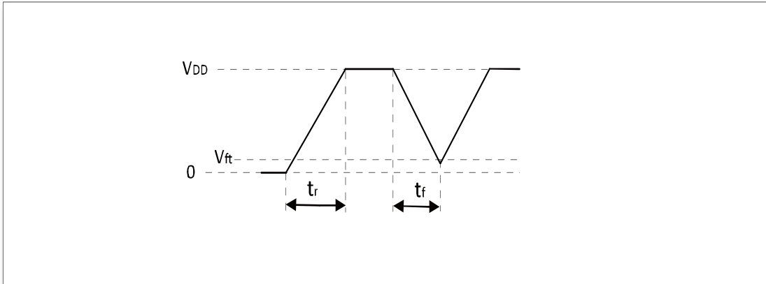
Figure 15 Power-up and power-down waveform
