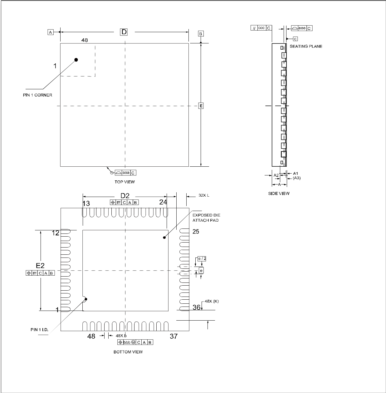
Figure 29 QFN48 low profile quad flat package
