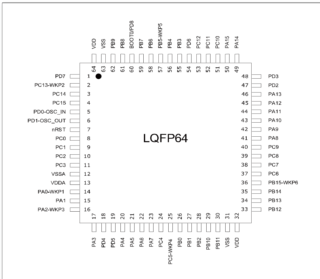
Figure 5 LQFP64 pinout diagram
