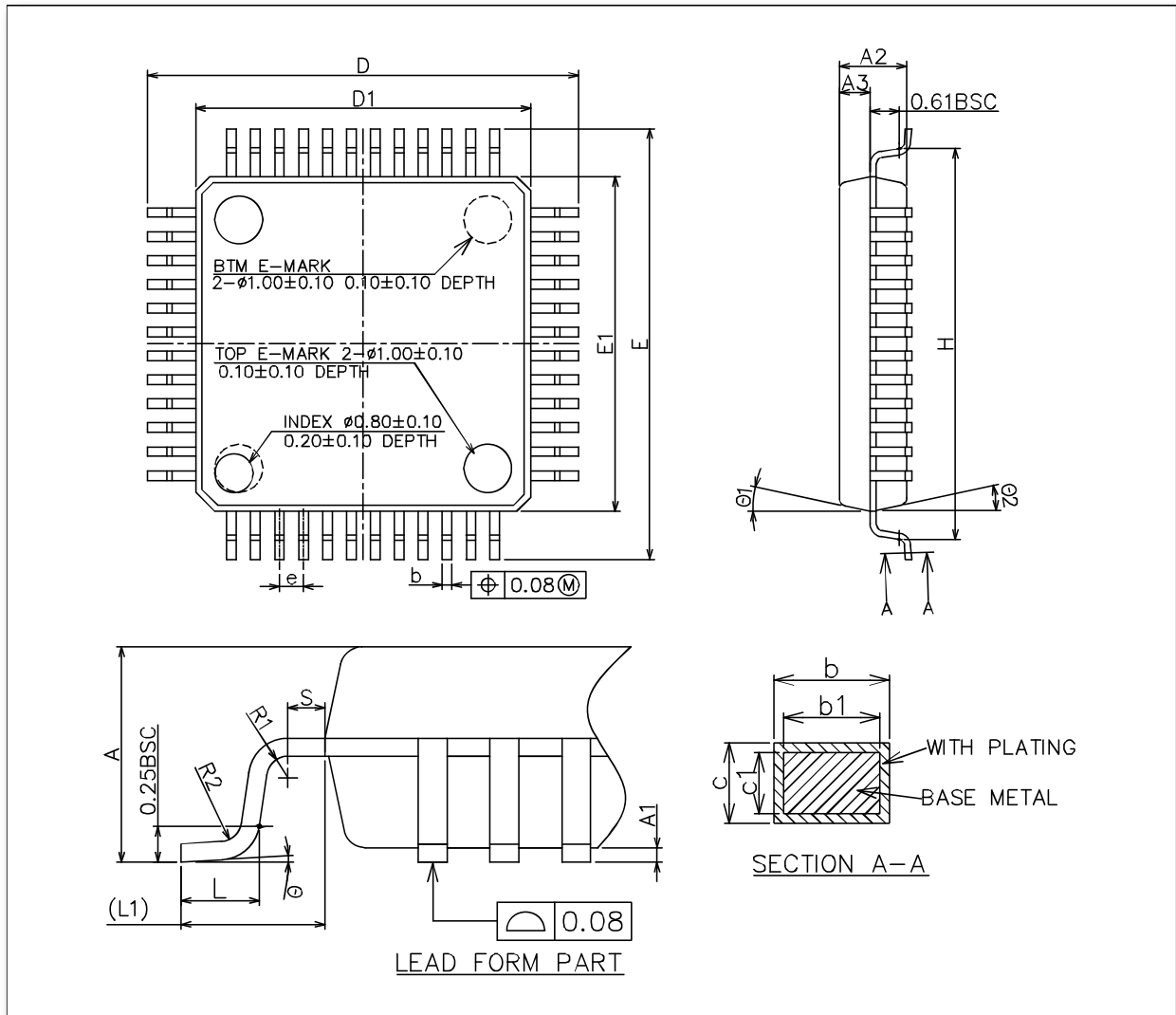
Figure 27 LQFP48, 48-pin low profile quad flat package
