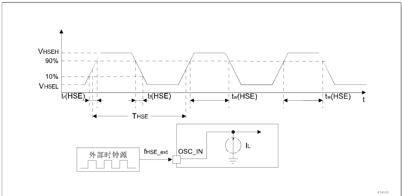
Figure 16 High-speed external user clock alternate current timing diagram
