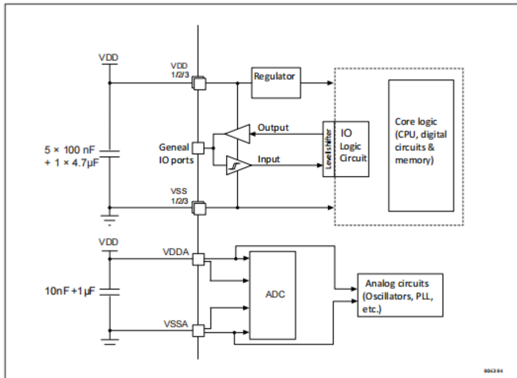
Figure 13 Power supply scheme
