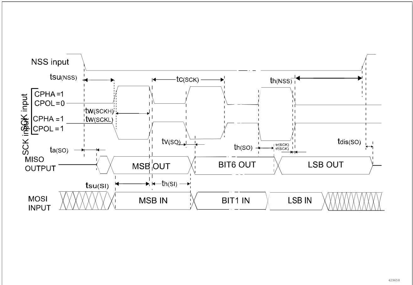
Figure 22 SPI timing diagram-slave mode and CPHA = 1, CPHASEL = 1 (1)
