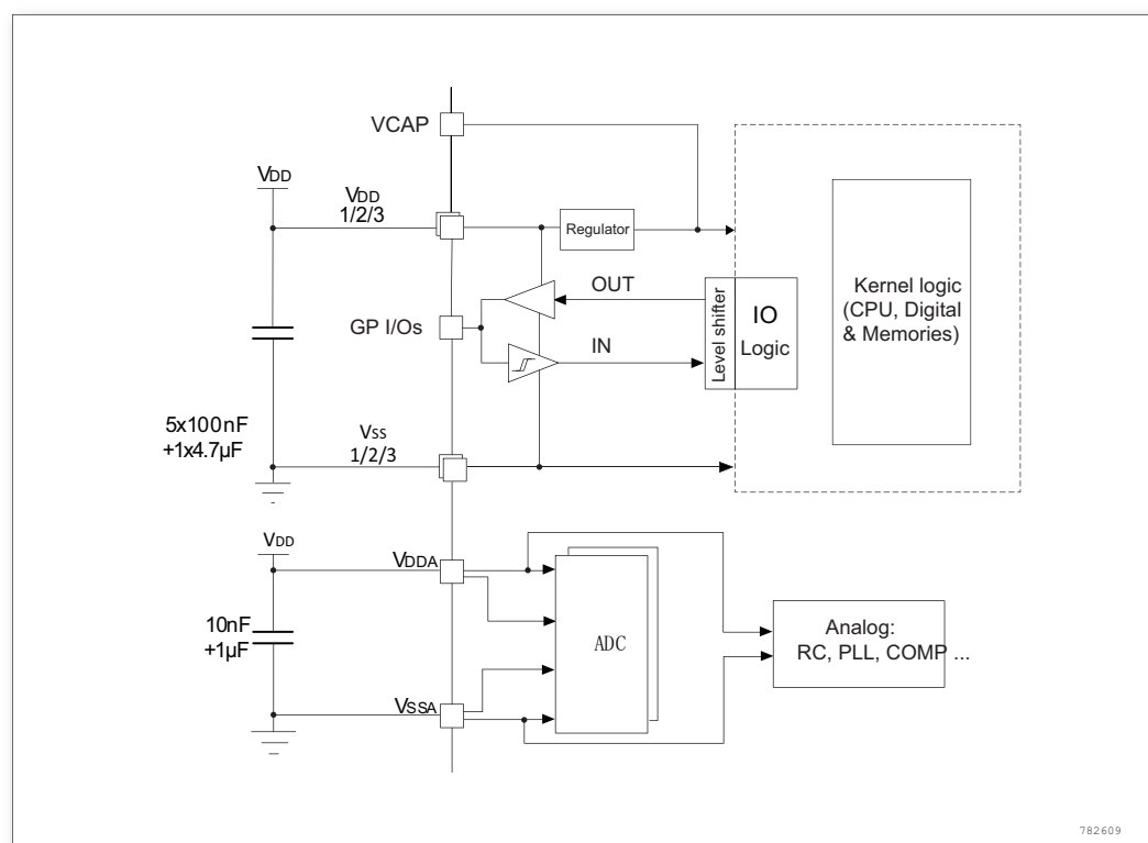
Figure 10. Power scheme
