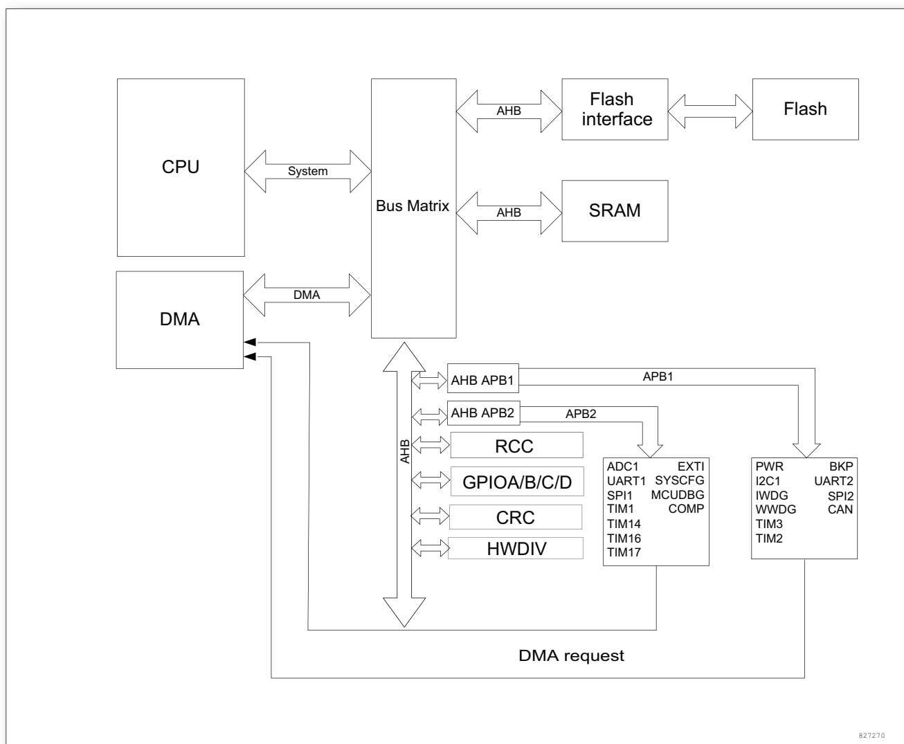
Figure 1. Block diagram
