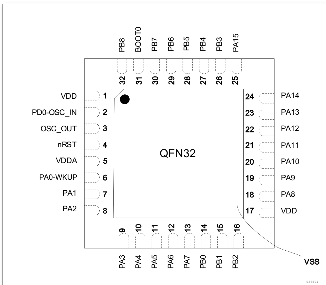
Figure 5. QFN32packet pinout
