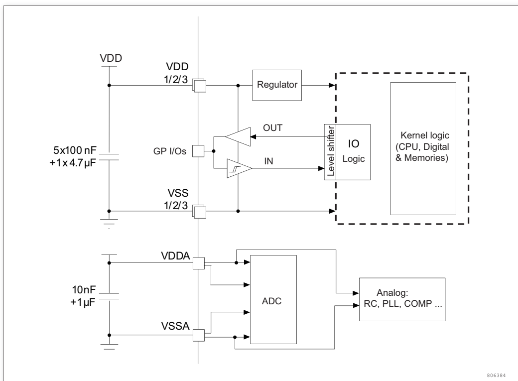
Figure 8. Power scheme
